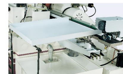
6. Automatic unloading attachment (thrufeed grinding)
